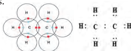
9.9. Electron-dot structure of ethane
