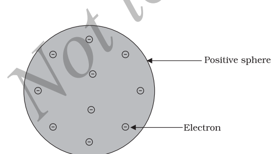
Fig.4.1: Thomson's model of an atom
