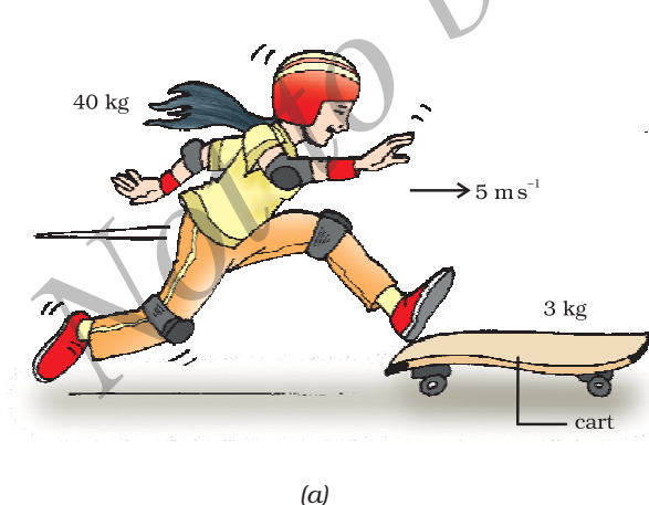
Fig. 9.18: The girl jumps onto the cart.
