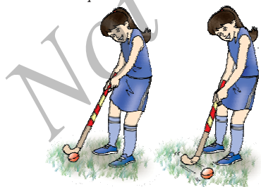
(c) The hockey stick hits the ball forward
