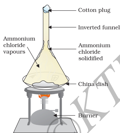
Fig. 1.7: Sublimation of ammonium chloride
